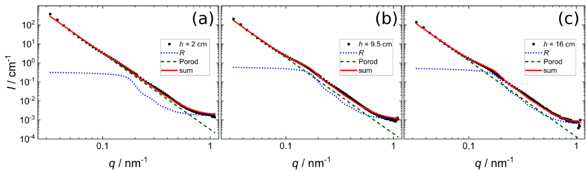
SANS data of a foam prepared from a 0.3 wt% dispersion of 2 mol% (BIS) cross-linked pNIPAM microgel, measured at different foam heights. (a) h = 2 \text{ cm} , (b) h = 9.5 \text{ cm} , (c) h = 16 \text{ cm} . Black squares are experimental data. For clarity the full curve (solid red line) is shown together with the Porod (dashed green line) and the reflectivity (dotted blue line) contribution.
